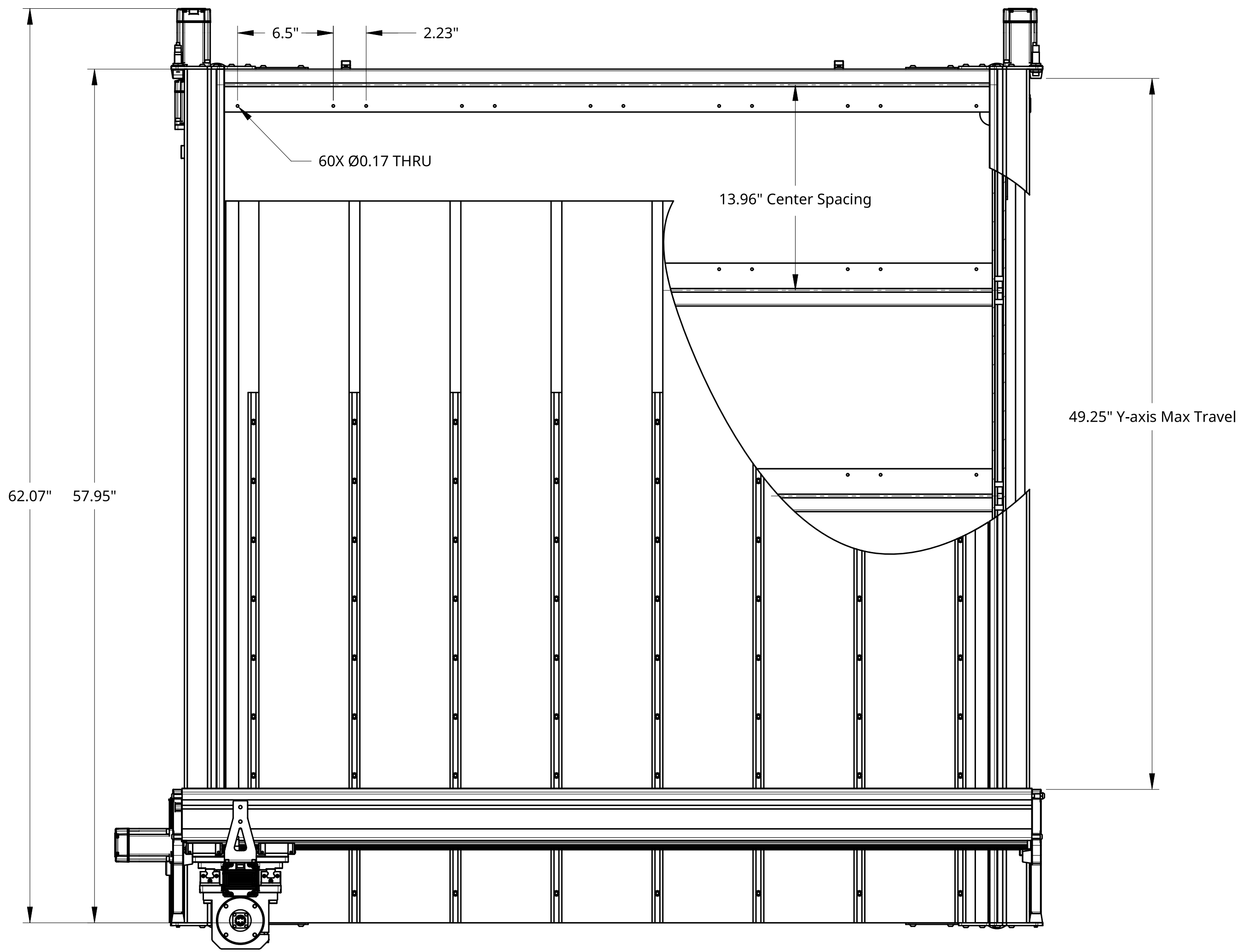
TOP VIEW
