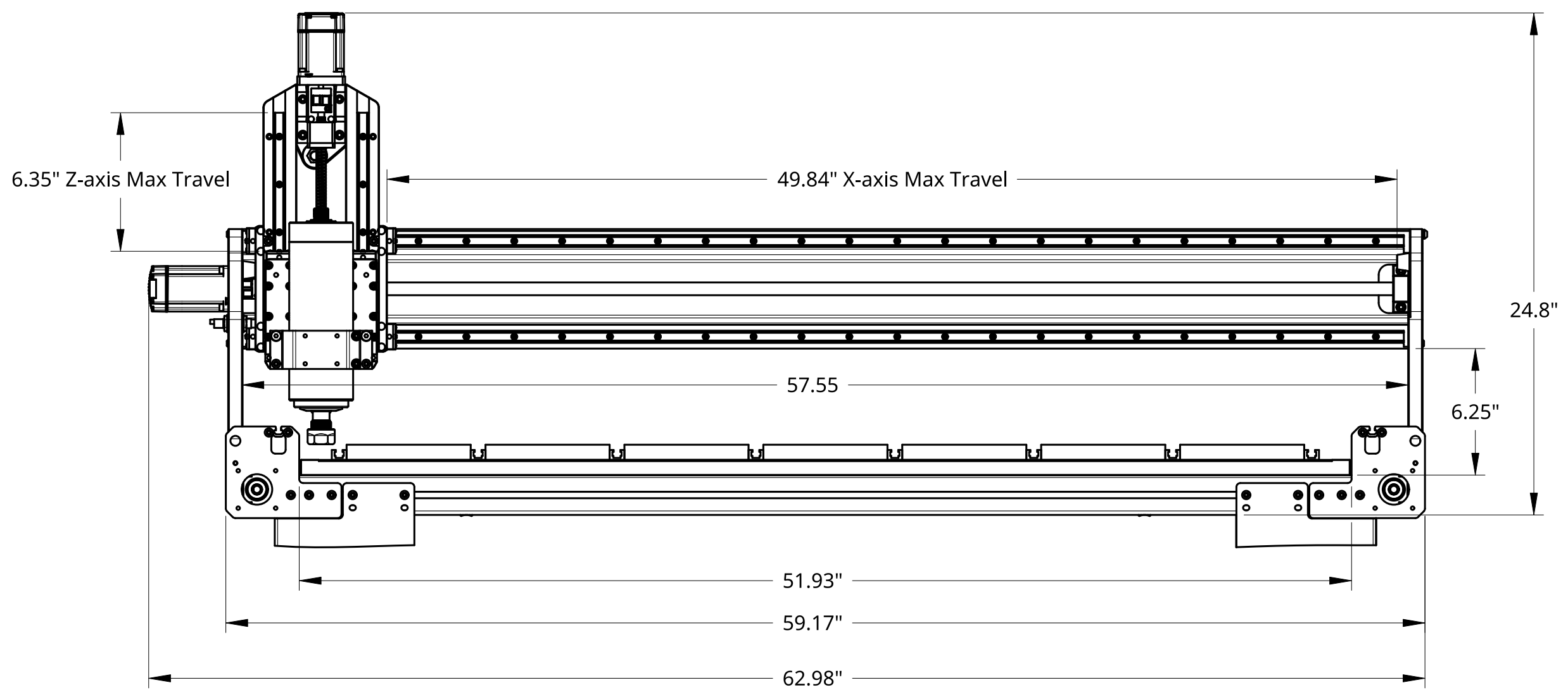
FRONT VIEW
