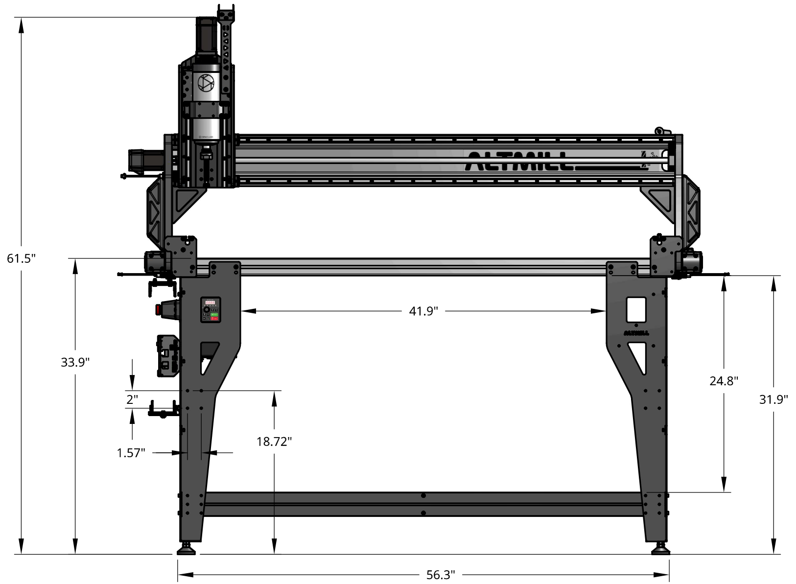
FRONT VIEW (Full Table)
