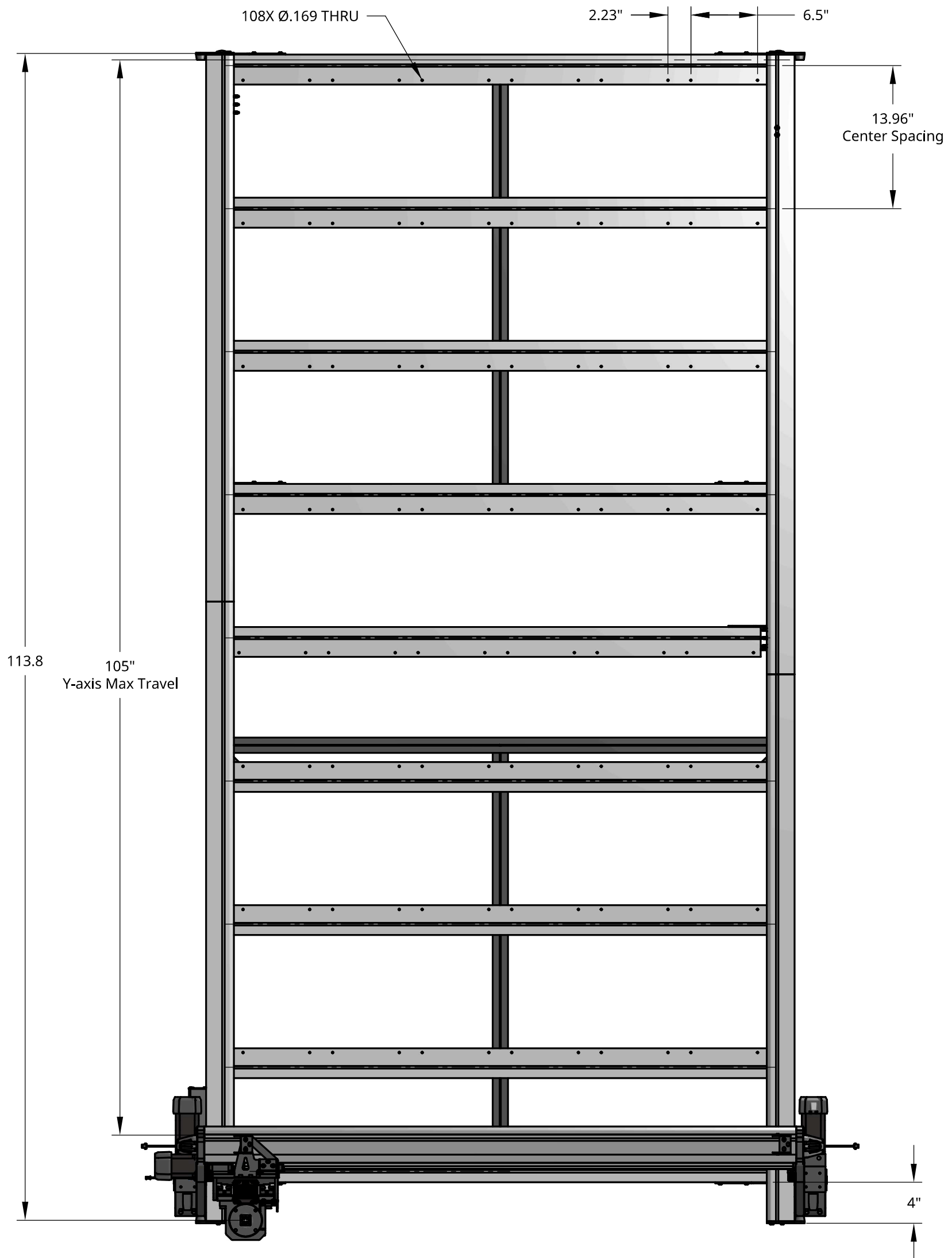
TOP VIEW (Joinery Configuration)
