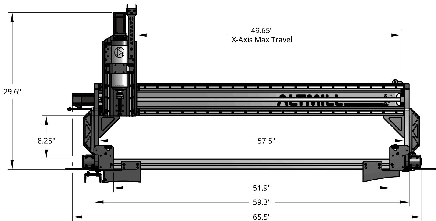
FRONT VIEW (Gantry View)
